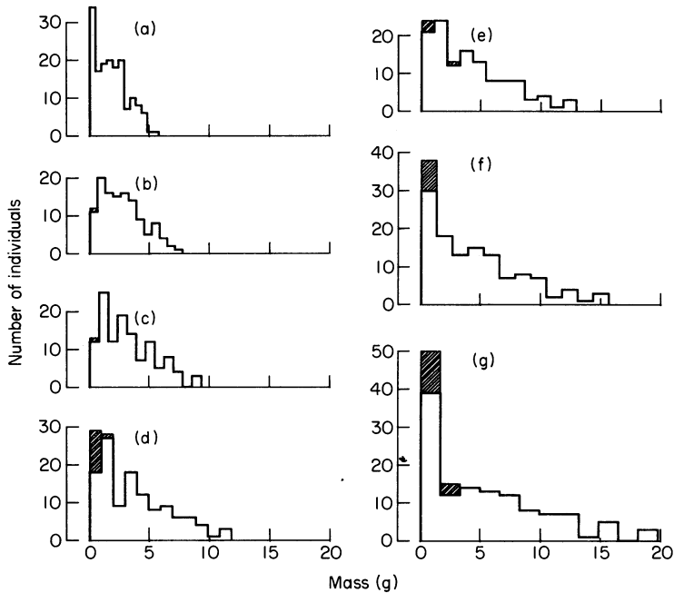
FIG. 4. Changing size distributions for an Impatiens pallida population in which individual fate was monitored weekly from (a) 23 July to (g) 11 September 1984. Initial and final distributions are based on direct size measurements. The intervening histograms are based on the assumption that individuals have linear growth (Fig. 2), and that individuals that subsequently died did not change in size (see text). Shaded columns represents individuals that died during a given time interval.
